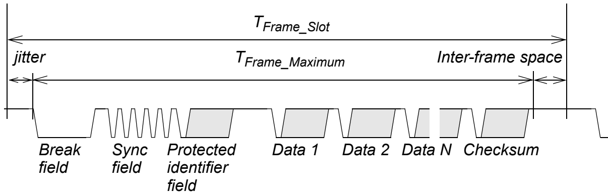
Figure 2.12: Frame slot
