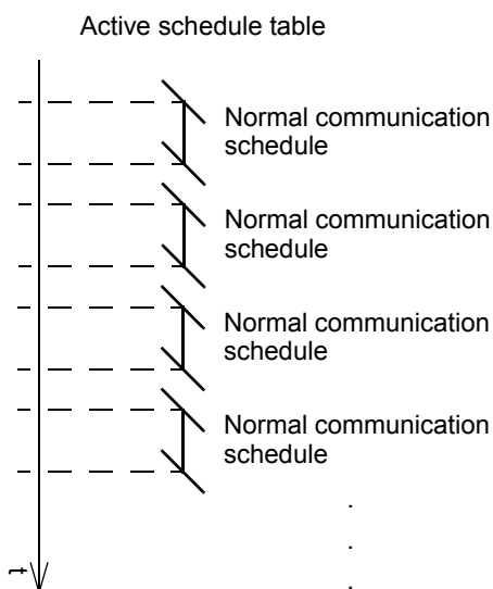
Figure 5.6: No diagnostic communication
