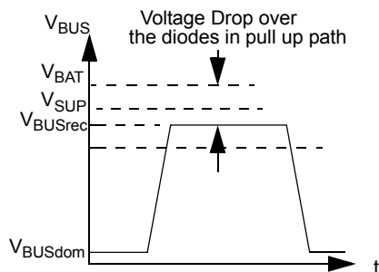
Figure 6.3: Illustration of the Difference between External Supply Voltage V_{BAT} and the Internal Supply Voltage V_{SUP}
