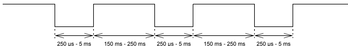
Figure 2.17: One block of wake up signals
